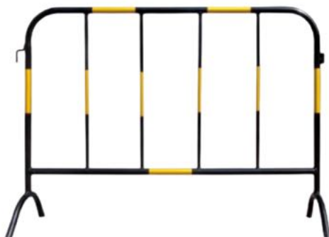
AEZB-1500-BK 1.5米黃黑鋅鐵圍欄 (單掛鉤) 尺寸: (L) 1500 x (H) 1000mm
