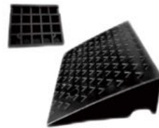
AESB-007 斜坡墊 尺寸:(L) 500 x (W) 350 x (H) 140mm (橡膠製)
