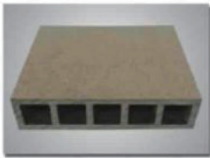
Deck (Hollow) Model: D140x22 Dimension(mm): 140X22
